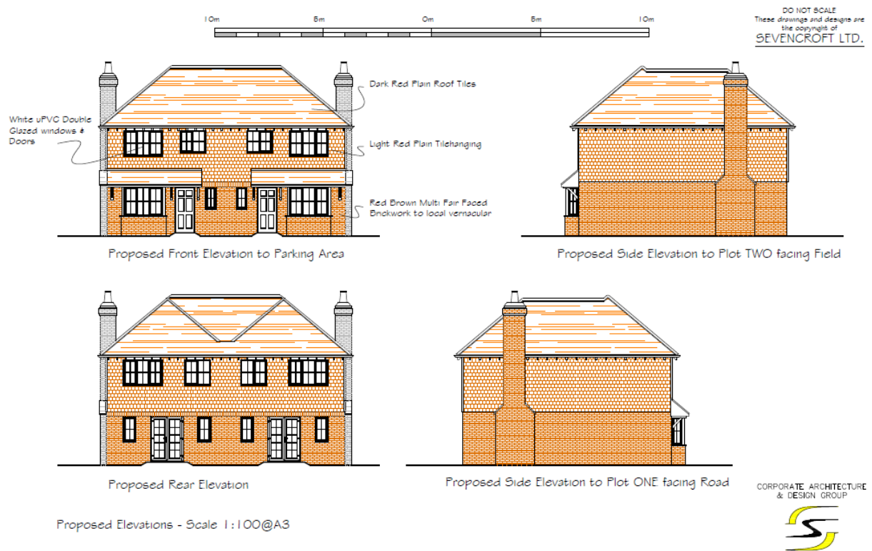
Figure 2 – Proposed Elevations
